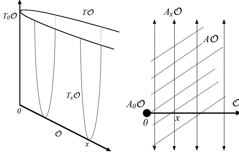
FIGURE 1. The tangent and admissible tangent bundles of example 41
